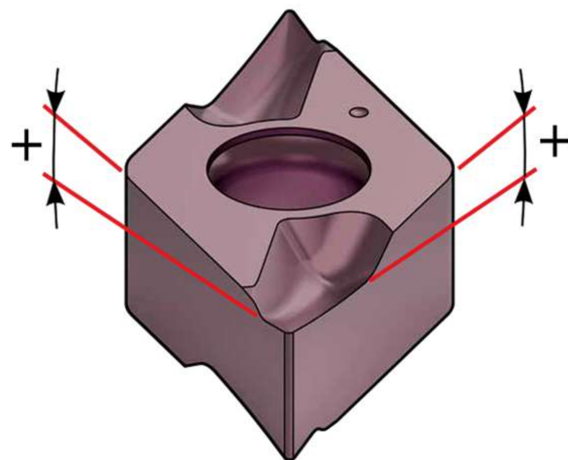
DNGX 130502M-ST-R Right hand insert
